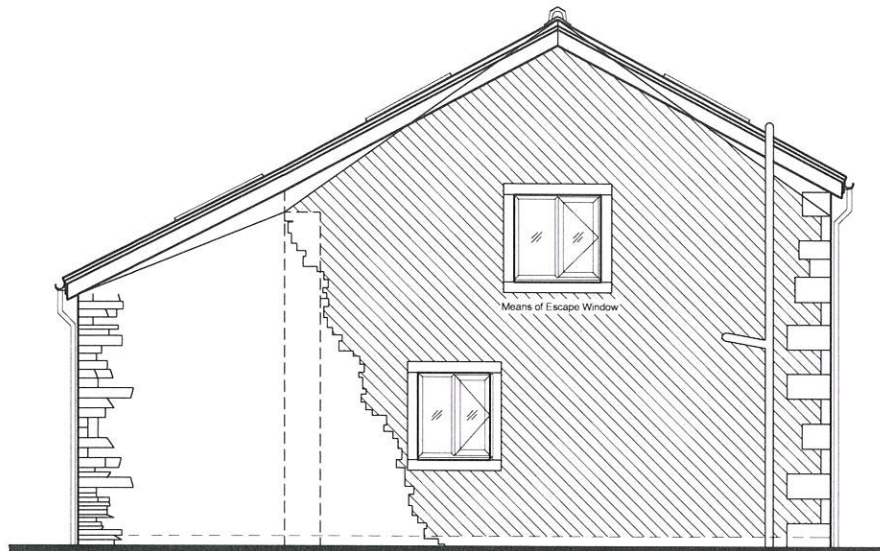
PLANNING APPROVED PROPOSED EAST ELEVATION
