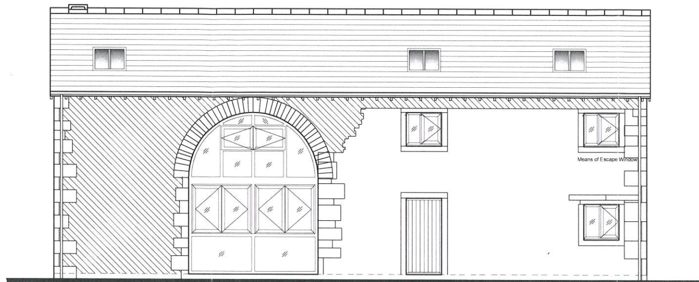
PLANNING APPROVED PROPOSED NORTH ELEVATION
